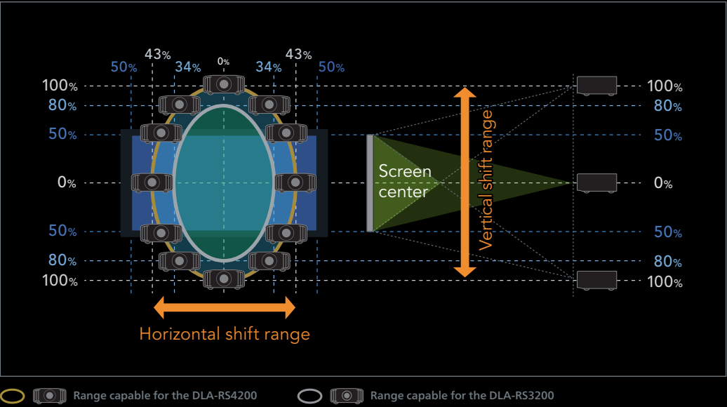
Above diagram shows shift range for the 16:9 aspect ratio projection.
